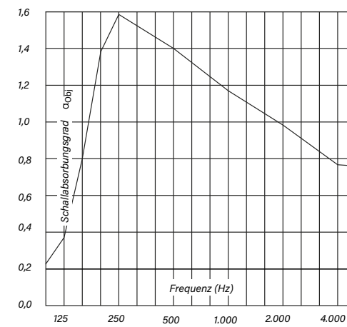
Schallabsorptionsgrad - Oktav-Mittenfrequenz (Eckabsorber)
